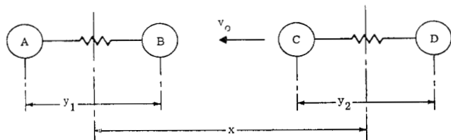
Figure 23. Collision model for AB + CD collisions. The distance between centers of mass is x and the internuclear distances are y_1 and y_2 .
