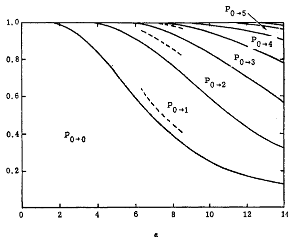
Figure 12. Transition probabilities vs. total energy out of the ground quantum state of an oscillator for m = 1/13 and \alpha = 0.1287 . The solid lines are the exact semiclassical results of Kerner and Treanor, and the dashed lines are the exact quantum results of Secrest and Johnson.
