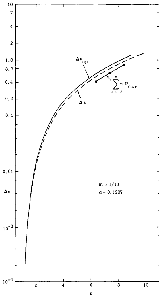
Figure 7. The energy transferred to an oscillator ( m = 1/13 and \alpha = 0.1287 ) as a function of total energy according to the approximate classical method ( \Delta\epsilon_{sp} ), the exact classical method for no initial excitation of the oscillator ( \Delta\epsilon ), and the exact quantum method for the oscillator initially in the ground quantum state ( \sum_{n=0}^{\infty} n P_{0 \rightarrow n} ) (initial oscillator energy of h\nu/2 ).
